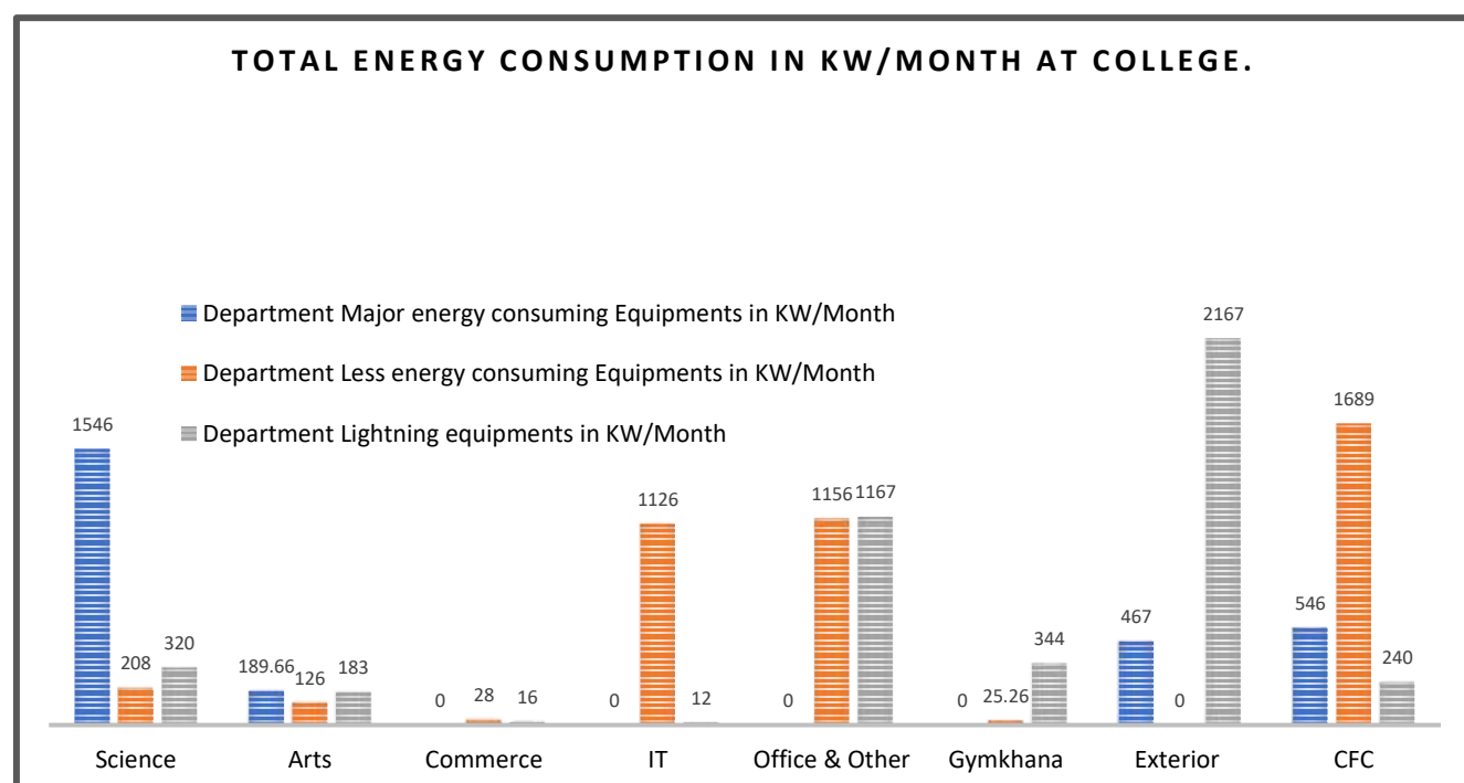
Graph No.1.4 Total energy consumption in KW/Month at college.
